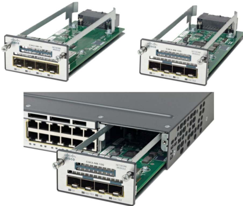
Figure 4. Network Module with Four GbE or Two 10GbE SFP+ Interfaces
